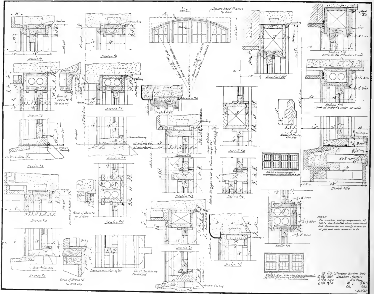
WOODEN WINDOW DETAILS
